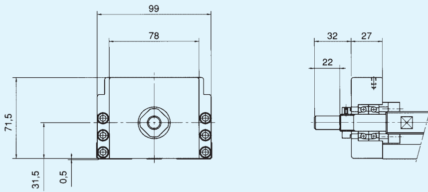
Abb. 10 KR55 Housing A ohne Motorflansch (Kennziffer □□10)
