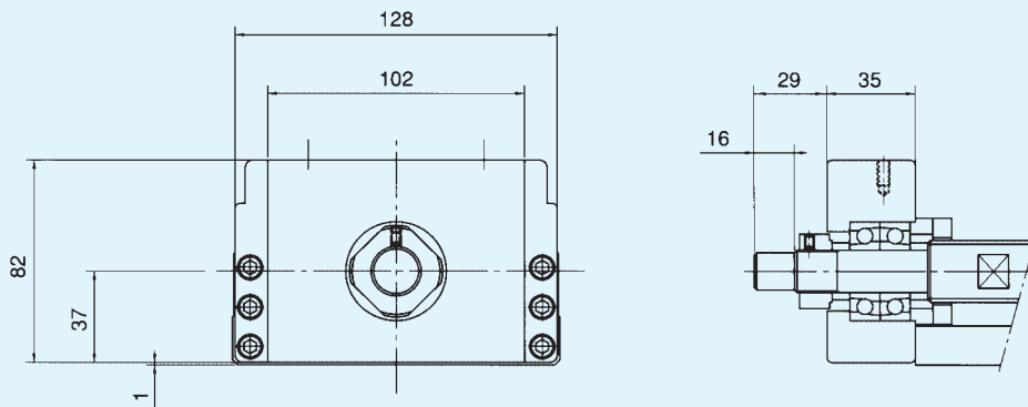
Abb. 11 KR65 Housing A ohne Motorflansch (Kennziffer □□10)
