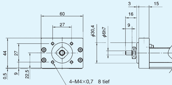
Abb. 7 KR33 Housing A ohne Motorflansch (Kennziffer 40)
