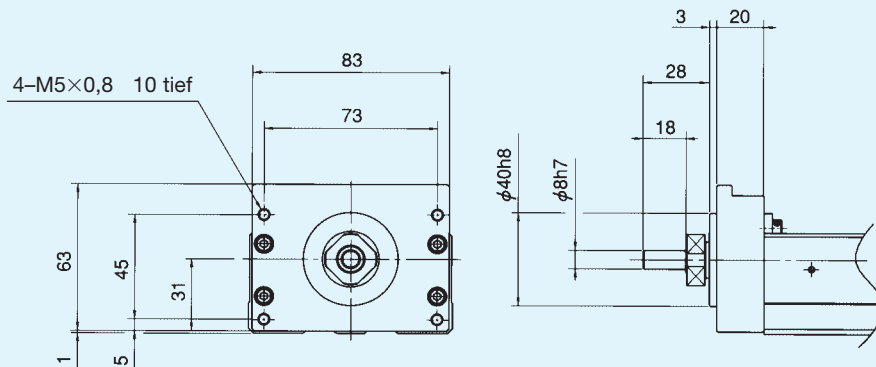
Abb. 8 KR46 Housing A ohne Motorflansch (Kennziffer 50)
