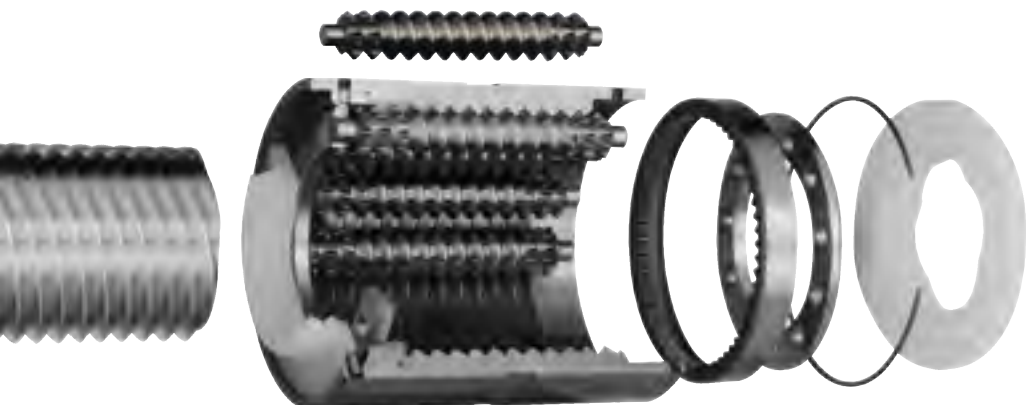
Threaded rollers are the basis of SR/BR/TR/PR planetary roller screws.
