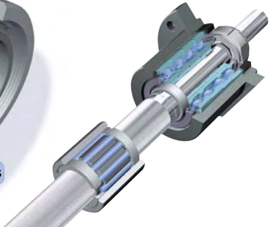
Recirculating roller screws
