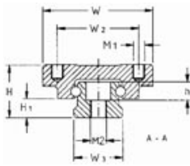
Main dimensions for miniature slide units
