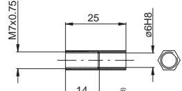
Connecting shaft SH
