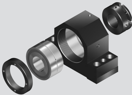
Pillow block unit SEB-F
