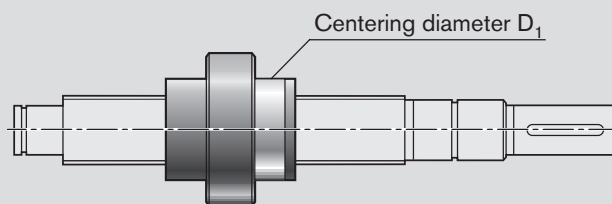
FEP-E-S Single nut with flange, Speed series
