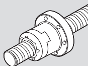
FSZ-E-S Single nut with flange, ECOplus series
