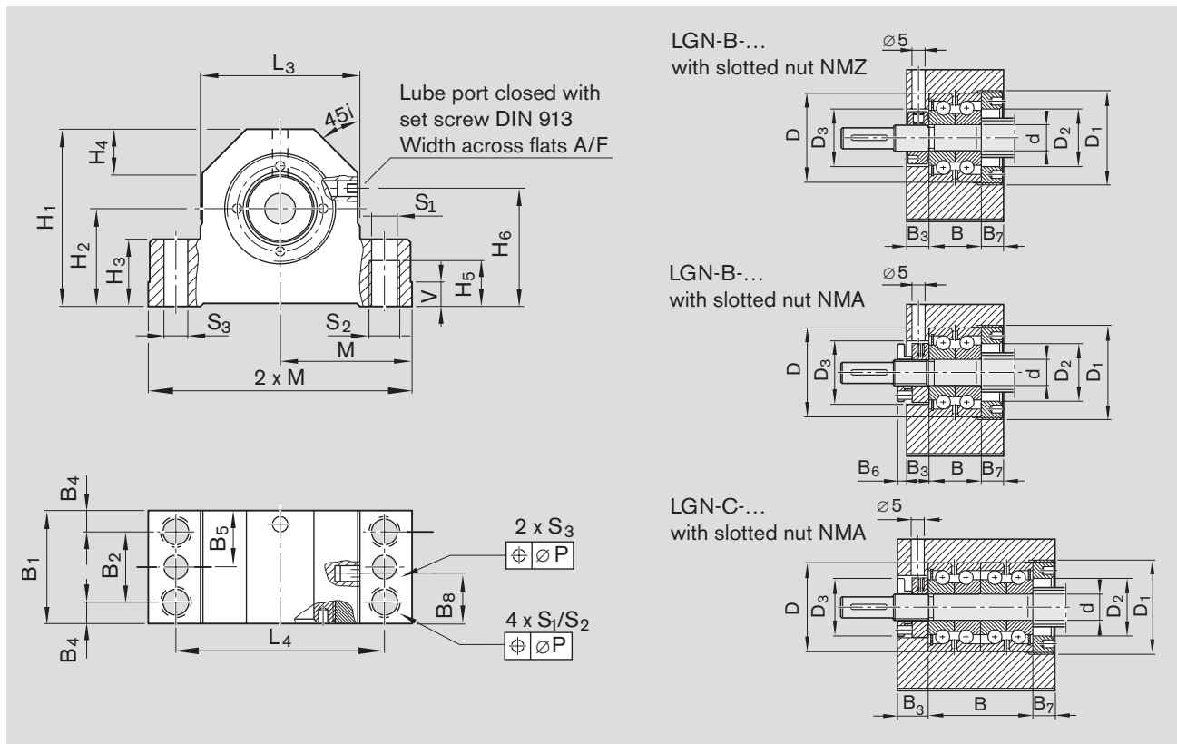
Dimensions (mm)
