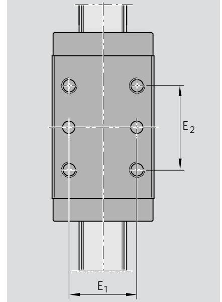
Runner Block Sxx
