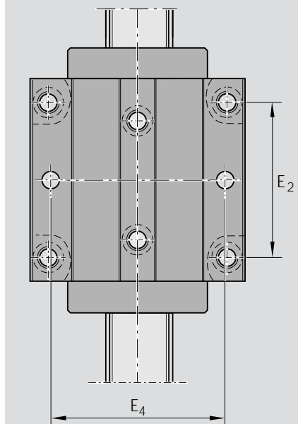
Runner Block Fxx
