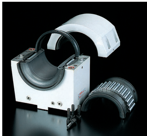
Photo 4 Split roller bearing units for segmented drive rolls
