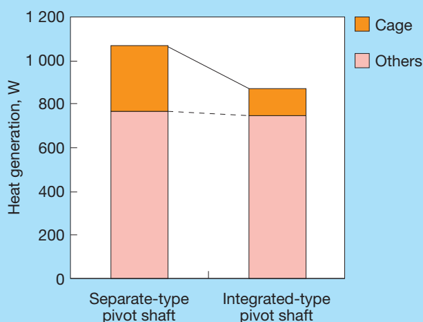
Fig. 7 Heat generation of power roller bearings when i=1.9 , n_{in}=2\,000\text{rpm} , T_{in}=350\text{N}\cdot\text{m}
