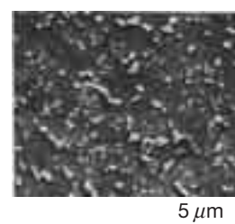
Photo 5. Microstructure of carburized conventional steel
