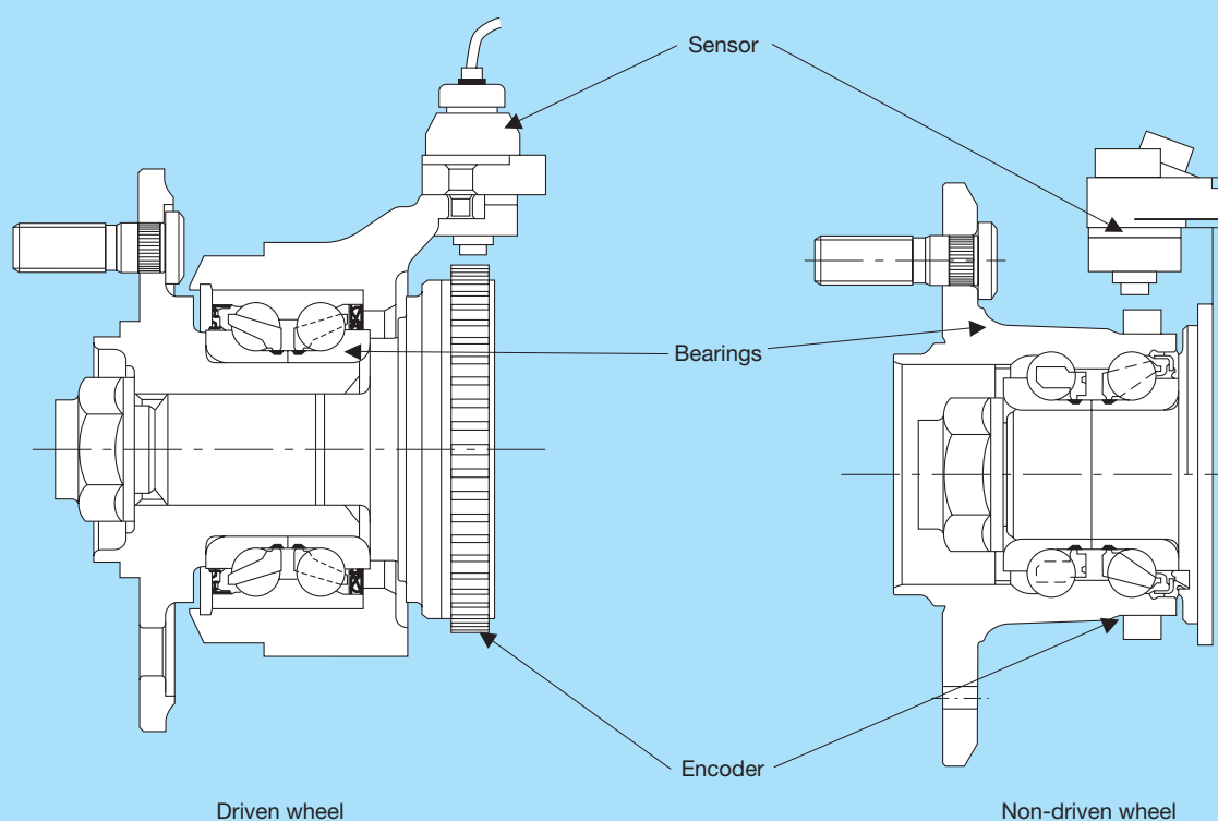
Fig. 7 Example of conventional hub units
