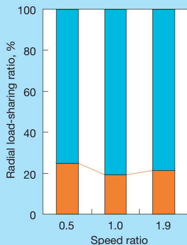
(a) Separate-type pivot shaft
