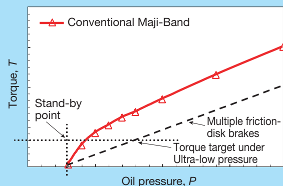
Fig. 4 Pressure and torque characteristics of a conventional Maji-Band
