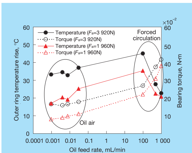
Fig. 10 Oil feed rate, frictional torque, and temperature rise of a ball bearing
