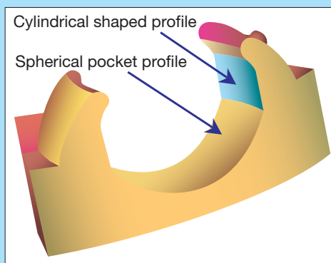
Fig. 3 Axial-cylindrical pocket cage
