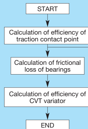
Fig. 10 Flow diagram for calculating half-toroidal CVT efficiency
