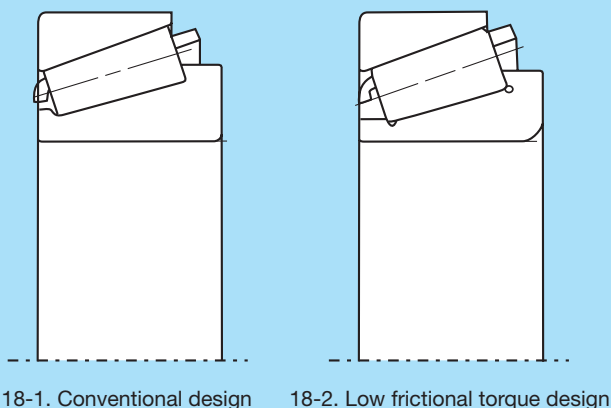
Fig. 18. Cross-section views of tapered roller bearings.
