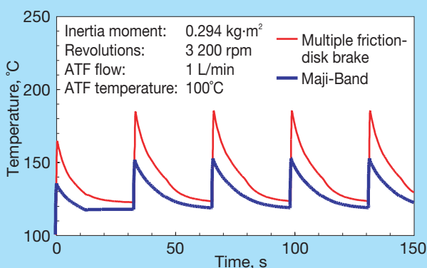
Fig. 3 Sliding surface temperatures of a multiple friction-disk brake and a Maji-Band
