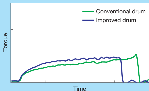
Fig. 10 Torque of the improved drum with surface treatment
