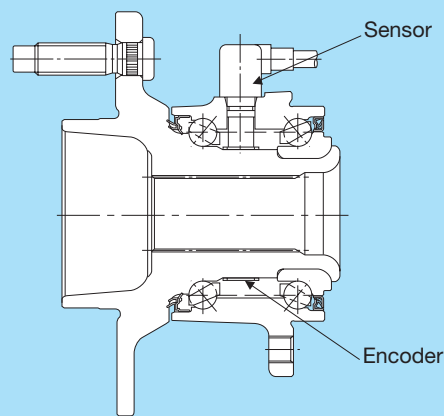
Fig. 10 Hub unit bearing with sensor unit between rows
