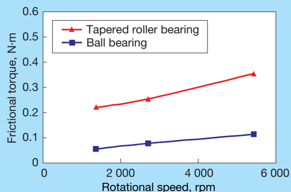
Fig. 19. Frictional torque comparison of tapered roller bearings and ball bearings
