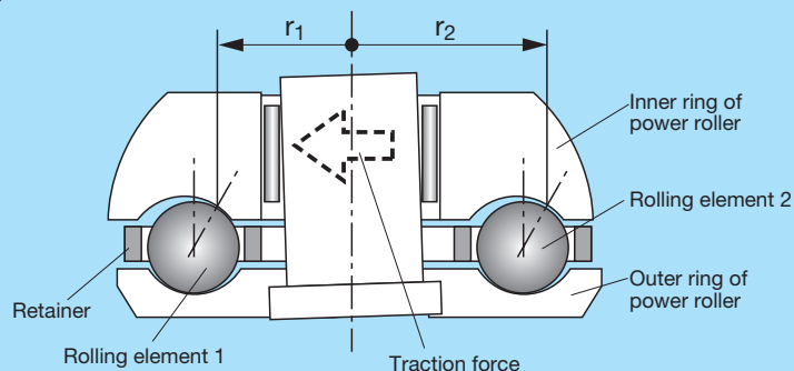
Fig. 8 Misalignment between the power roller inner and outer rings
