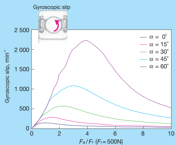
Fig. 6 Gyroscopic slip of a ball
