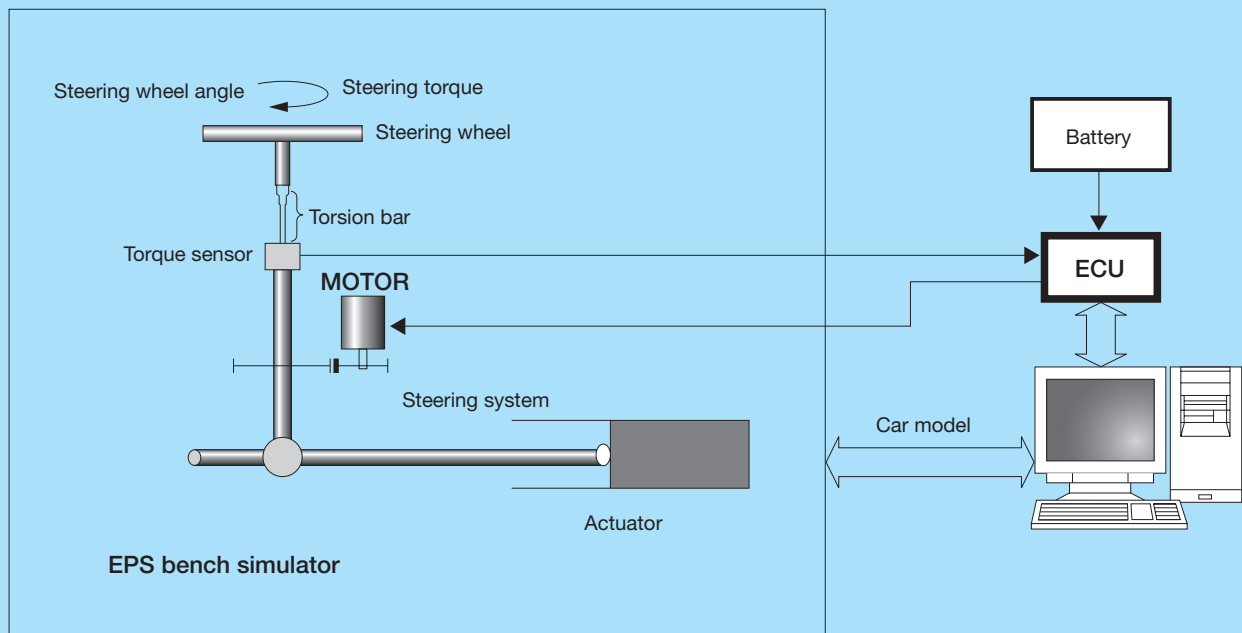
Fig. 9 Driving simulator
