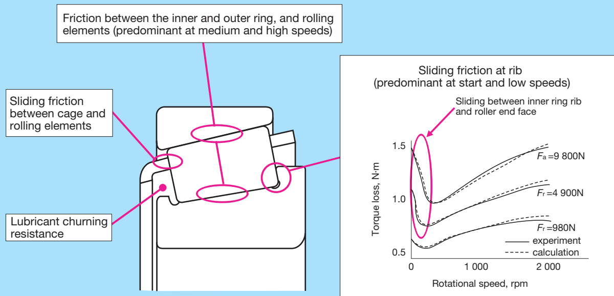
Fig. 2 Friction areas of a tapered roller bearing
