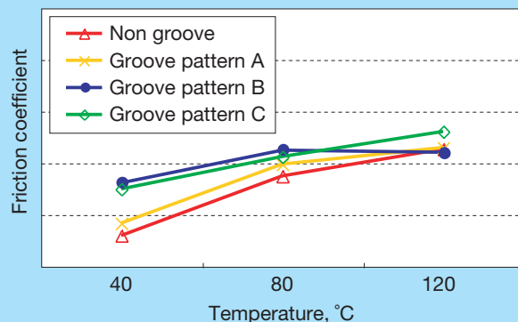
Fig. 11 Improved temperature dependency for different groove types.
