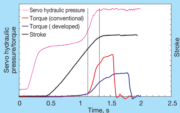
Fig. 13 Band torque for stroke using servo piston
