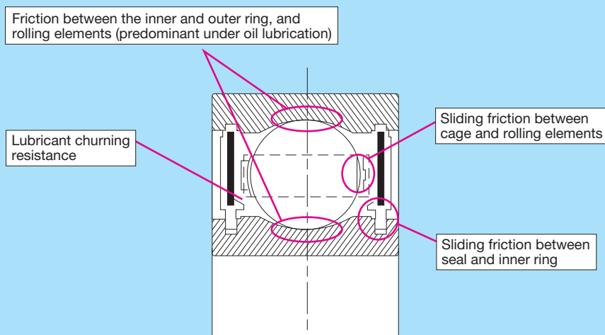
Fig. 1 Friction areas of a ball bearing
