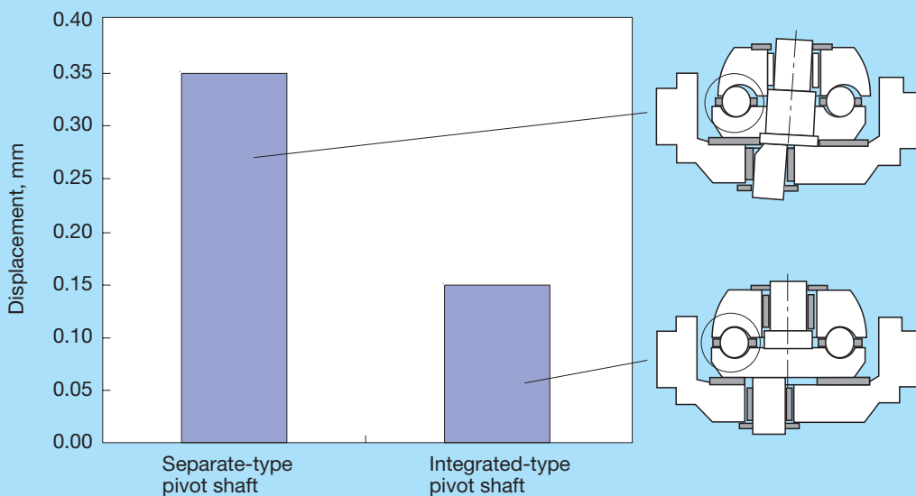
Fig. 3 Amount of inner ring displacement for both types of pivot shaft under F_r = 2\,000\text{N}
