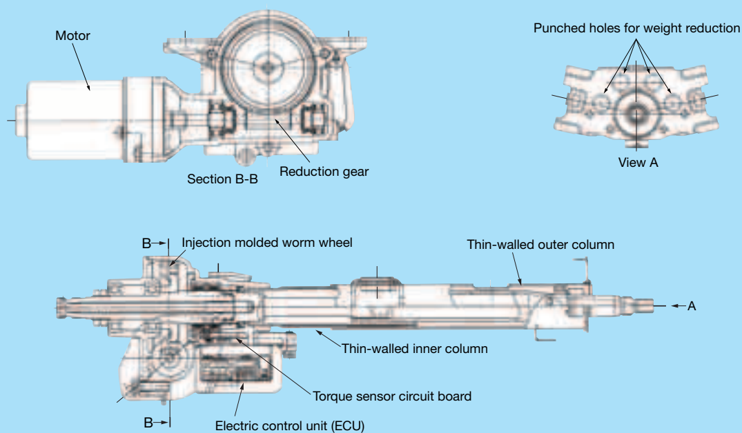
Fig. 1 Construction of column type EPS
