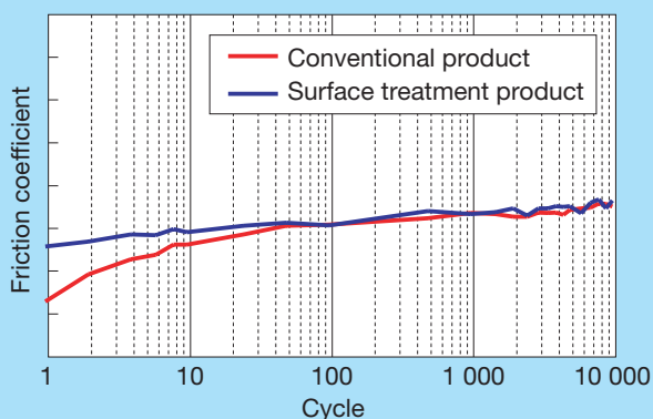
Fig. 12 Break-in behavior of developed Maji-Band
