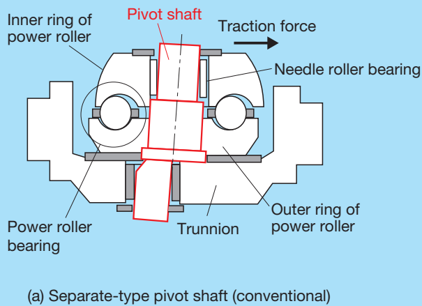
Fig. 2 Separate type and integrated type of pivot shaft
