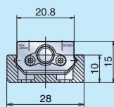
MCM02 Mass: 0.26 kg (Stroke: 50 mm)
