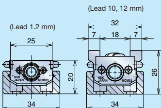
MCM03 Mass: 0.7 kg (Stroke: 100 mm)
