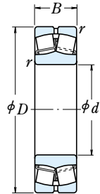
Cylindrical Bore
