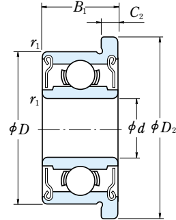
Shielded Type ZZ · ZZ1
