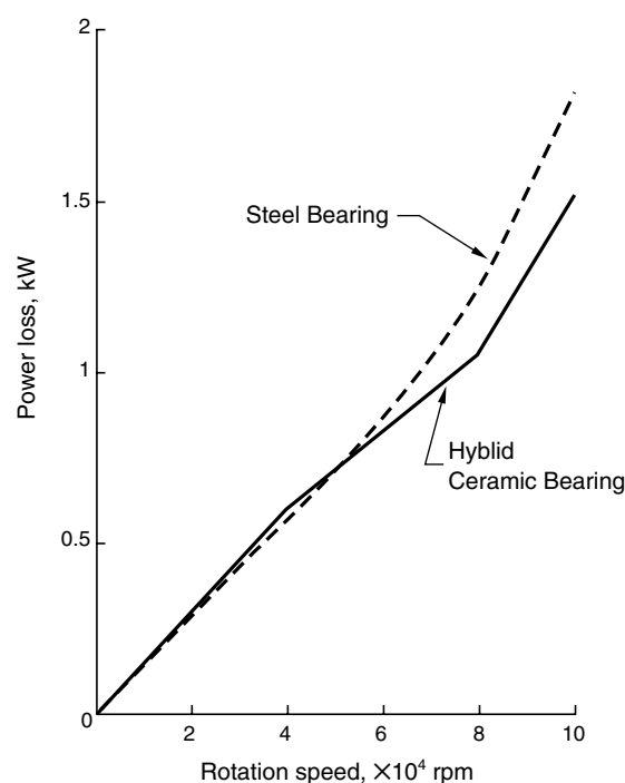
Fig. 2.5 Comparison of Power Loss between Hybrid Ceramic Bearing and Steel Bearing
