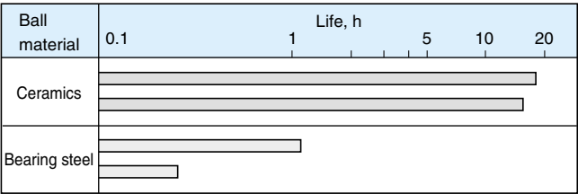
Fig. 4.11 Seizure Life Test Results for Hybrid Ceramic Ball Bearings
