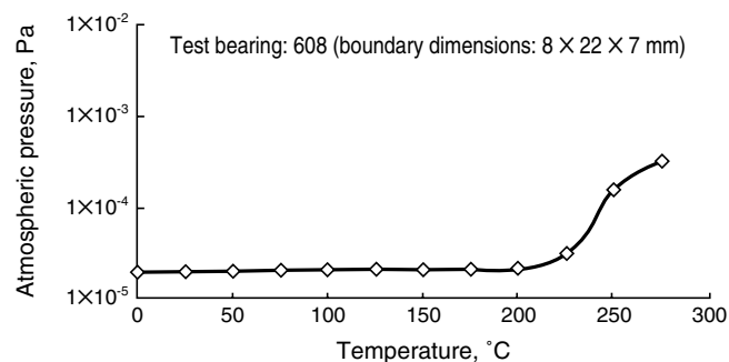
Fig. 3.7 Pressure Changes when Bearing Coated with Special Polymeric Fluoride Is Heated
