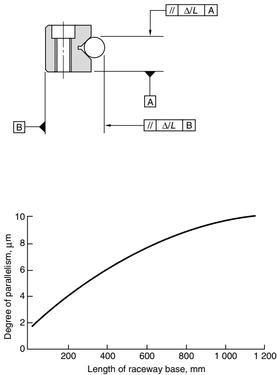
Fig. 9.3 Degree of Parallelism of Raceway Surface of Cross Roller Way Bearing Unit
