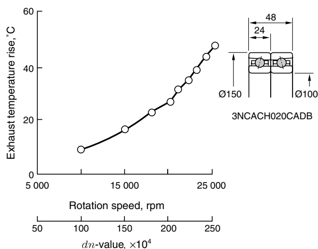
Fig. 4.4 ③ High-speed Performance Test Result for Hybrid Ceramic Ball Bearings (Jet Lubrication)
