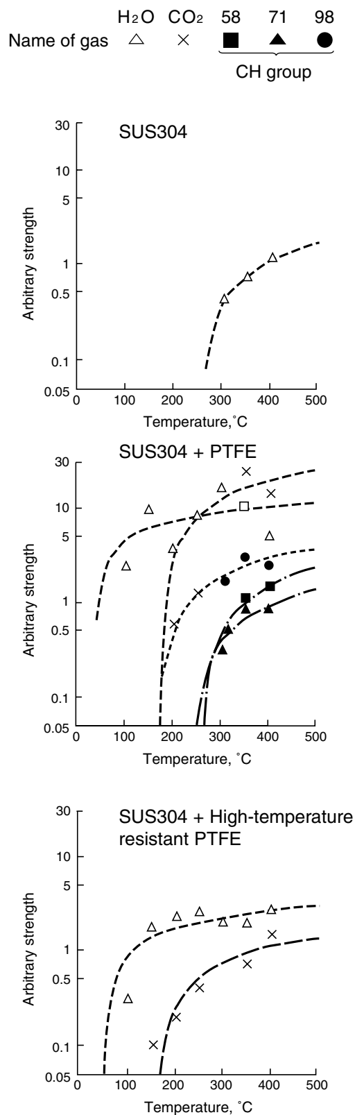
Fig. 3.6 Type of Gas Emitted from Heated Retainer
