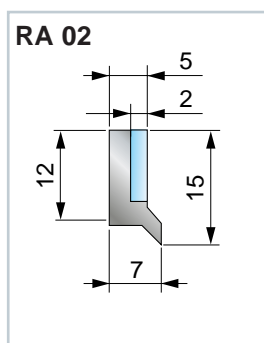
Profile: Synthetic rubber Length: 560 mm Steel insert
