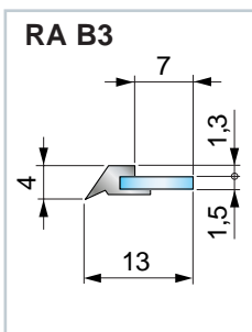
RA B3 Profile: Synthetic rubber Length: 560 mm. Steel insert
