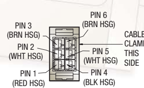
C2 BRAKE SWITCH SEPARATE CIRCUIT
