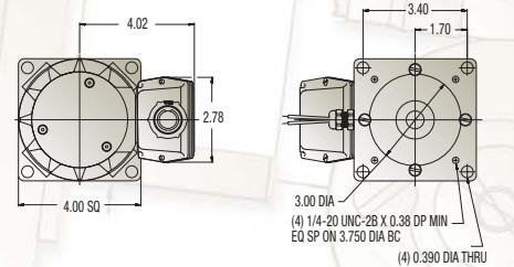
MOTOR TACHOMETER OPTIONS SHOWN: SQUARE MOUNTING, JUNCTION BOX, SEALED
