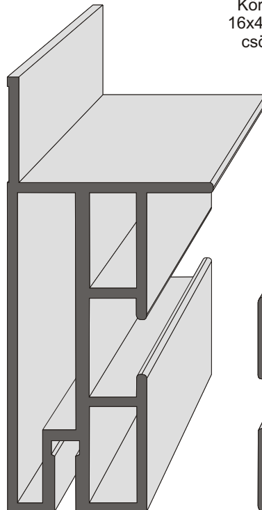
HA02 Keretprofil 90,20 x 43,50 mm HL=6100 mm
