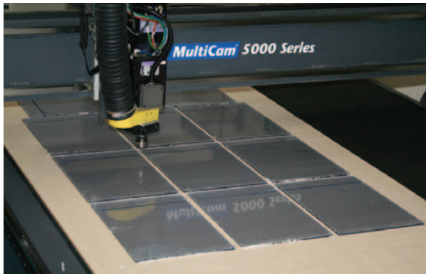
Fabrication of plastics for equipment production on 2m x 3m CNC Machine.
