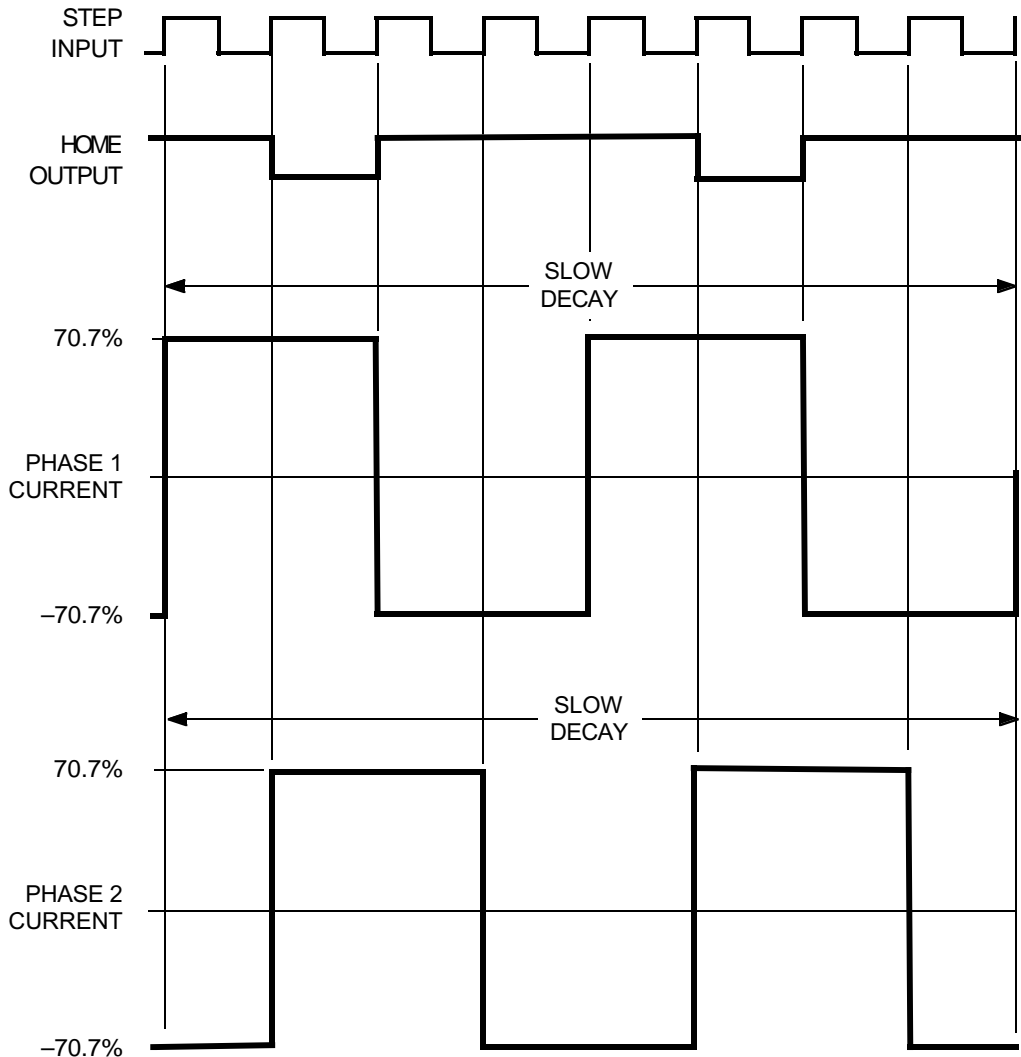
Full-Step Operation MS_1 = MS_2 = L, DIR = H
