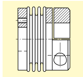
Series AKD/CK Model with clamping hub and flange
