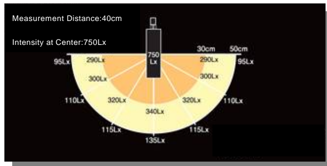
Illumination distribution
