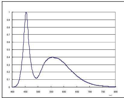
Emission Spectrum
