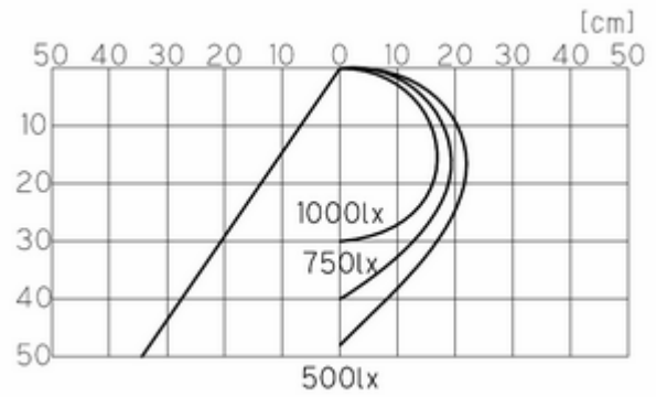
Luminous Intensity distribution
