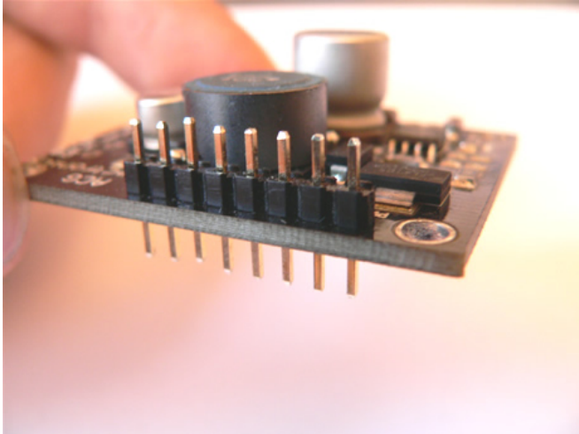
ACG-D1000 with I-header (longer leg size can be achieved by attaching from bottom)
