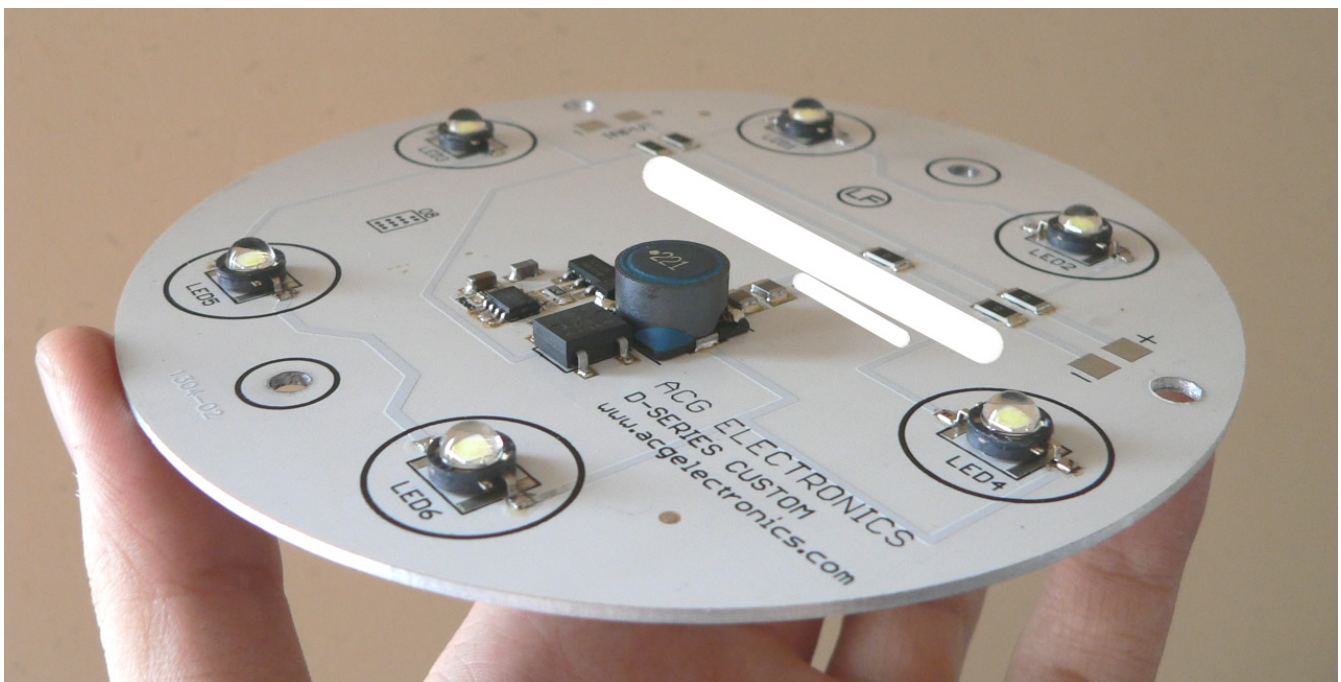
D-Series custom0018v4 – custom production LED module with integrated D-Series constant current driver-
