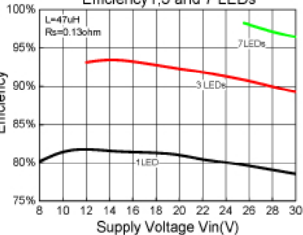
Efficiency 1,3 and 7 LEDs
