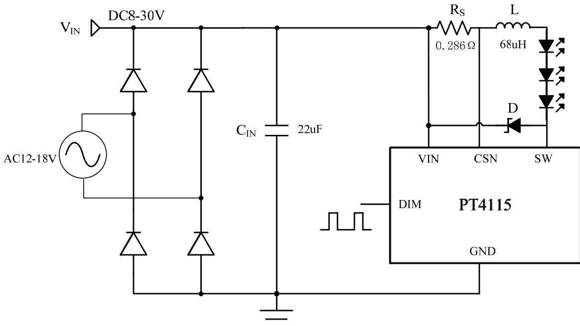
Fig 2: 3W application
