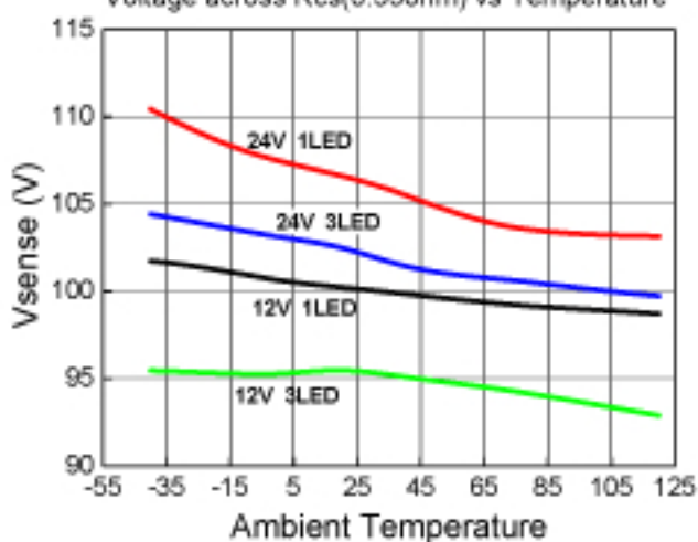
Voltage across Rcs(0.33ohm) vs Temperature
