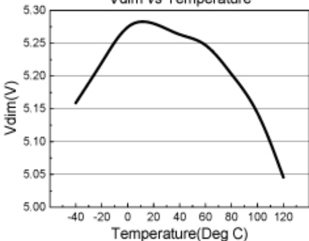
Vdim vs Temperature
