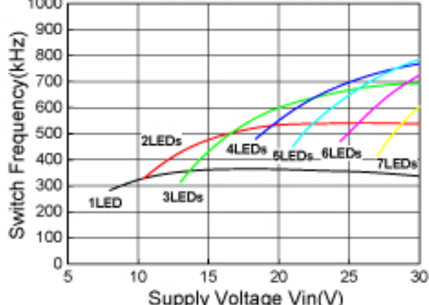
Switch Frequency L=100\mu\text{H} R=0.33\text{ohm}
