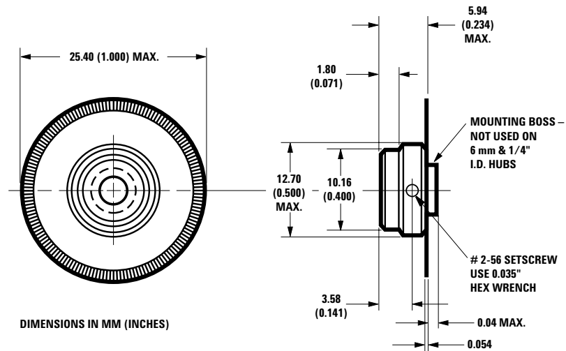
Figure 4. HEDS-5120 Codewheel.
