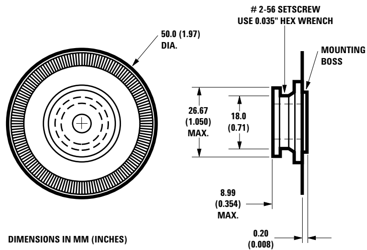
Figure 5. HEDS-6100 Codewheel.
