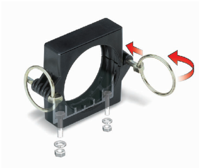
Mounting Brackets
