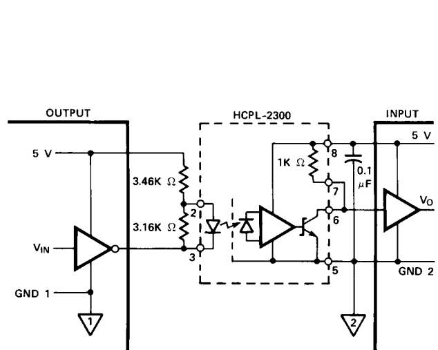
Figure 14. Series Drive from Open Collector TTL/LSTTL Units.
