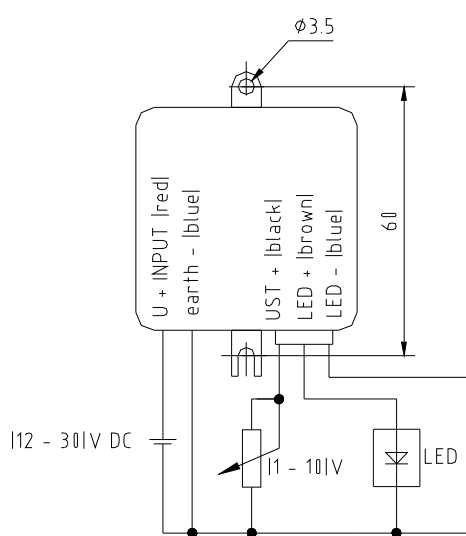
Connecting diagram LED drive-35 / 70 DC
