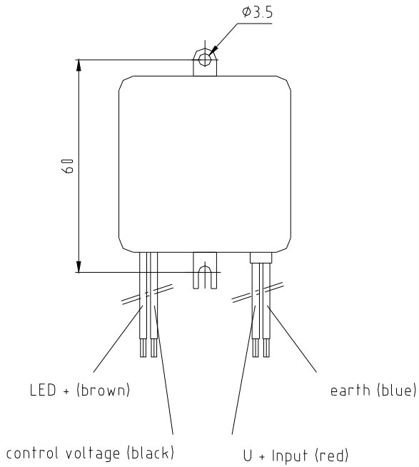
Closed housing with connecting leads
