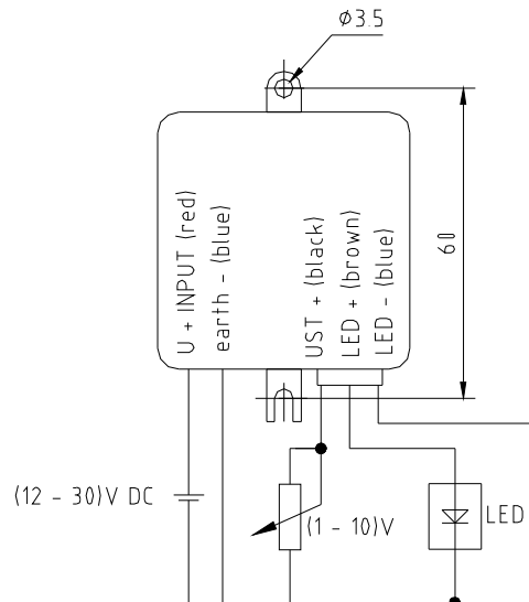
Connecting diagram LED drive - 100 DC
