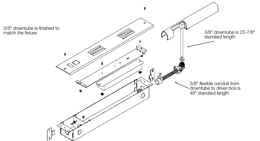
Type F Wiring Option: downtube
