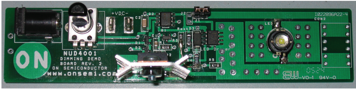
Figure 7. Demonstration Board Built with the Dimming Circuit, the External Transistor, and an Onboard LED
