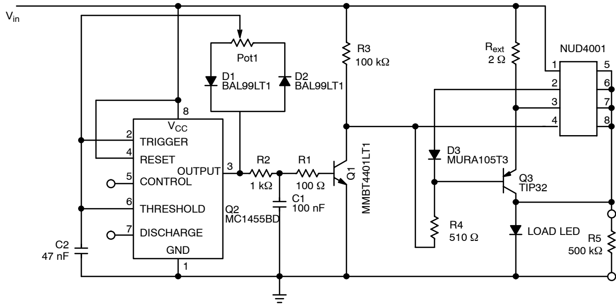
Figure 1. PWM Circuit Diagram
