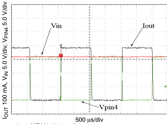
Figure 3. Circuit Behavior at ~50% Duty Cycle
