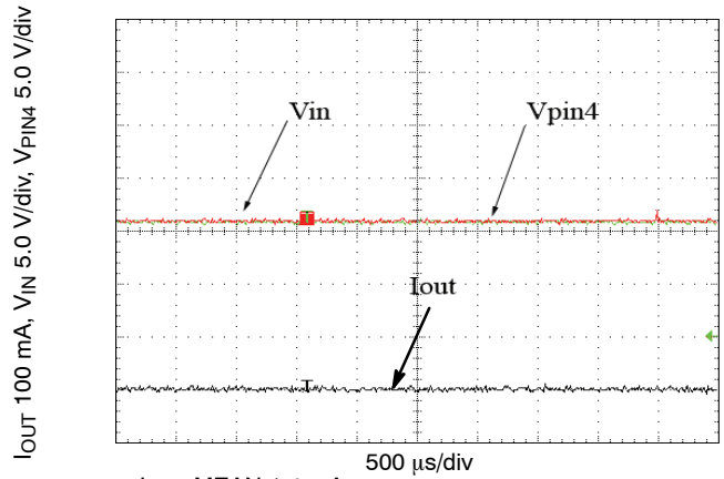
Figure 4. Circuit Behavior at 0% Duty Cycle
