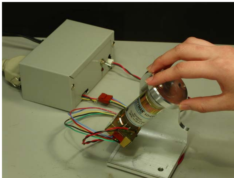
Figure 1. The Twiddler and Electronic Box Shown in Operation
