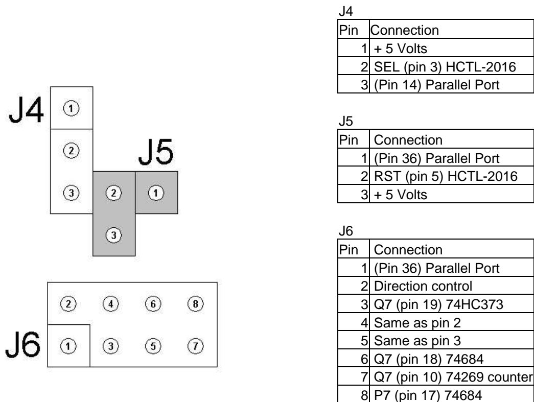
Figure 10. Jumper Locations
