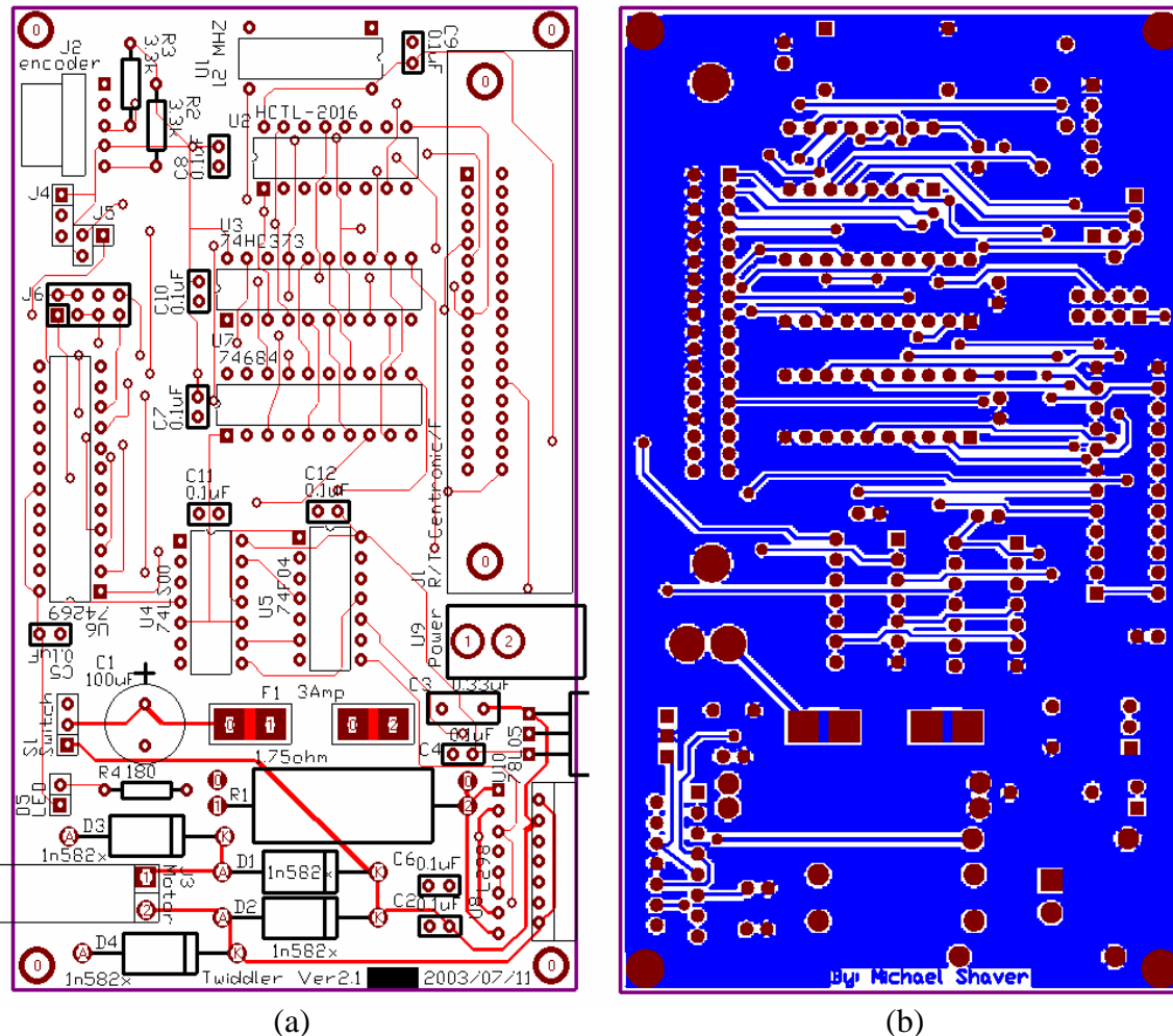
Figure 8. Twiddler Version 2.1 Printed Circuit Board (a) Top of PCB, traces in red (b) Bottom of PCB (flipped along long edge), Traces in Blue
