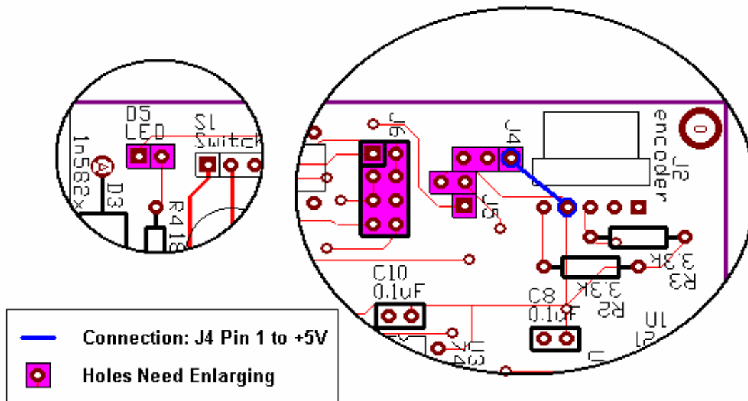
Figure 9. Corrections Required on Existing Blank Version 2.0 Boards
