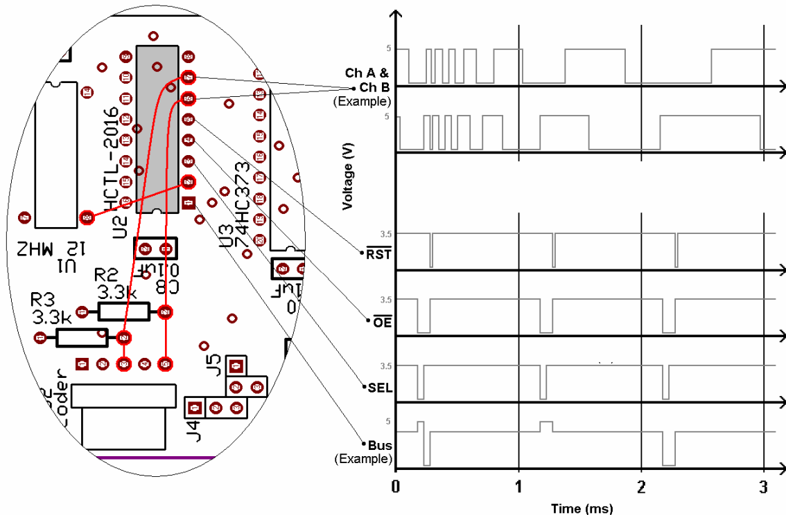
Figure 17. Expected Signals From Encoder Input Hardware
