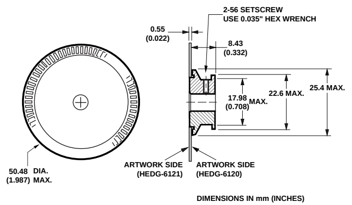
Figure 11. HEDG-6120 Codewheel/HEDG-6121 Codewheel.
