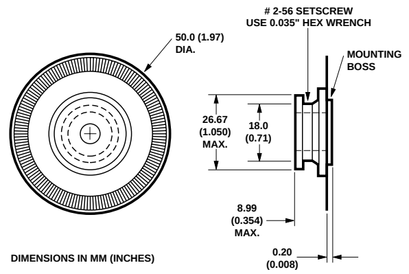
Figure 5. HEDS-6100 Codewheel.
