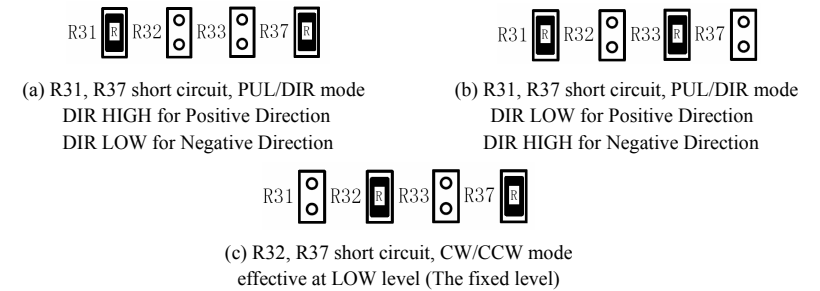
Figure 2: PUL/DIR and CW/CCW settings
