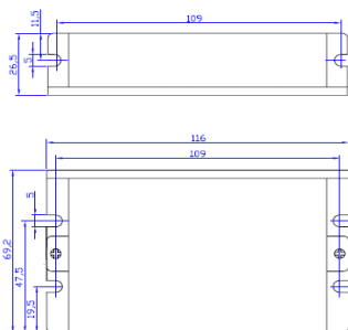
Figure 1: Mechanical specifications
