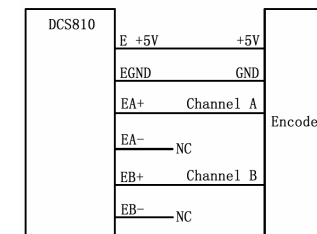
Figure 7: The DCS810 supplies the single-ended encoder directly
