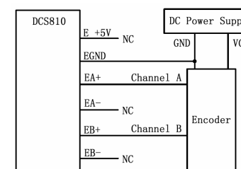
Figure 9: Using external DC power supply to supply the single-ended encoder
