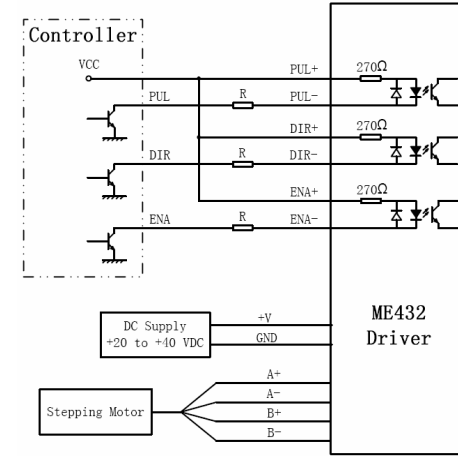
Figure 10: Typical connection
