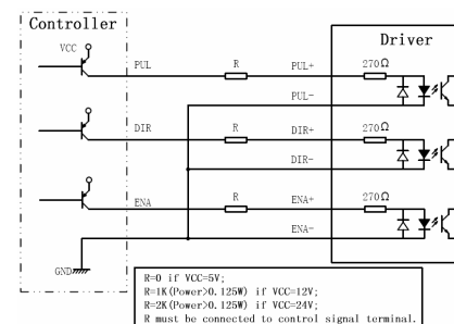
Figure 4: Connection to PNP signal (common-cathode)
