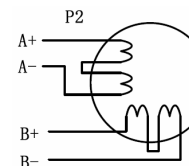
Figure 8: 8-lead motor series connections
