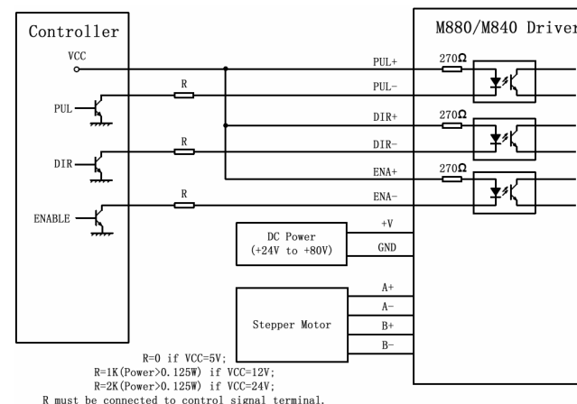
Figure 10: Typical connection
