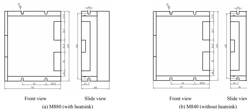
Figure 1: Mechanical specifications
