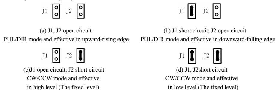
Figure 2: J1 and J2 jumpers
