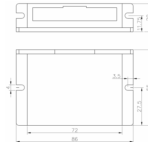
Figure 1: Mechanical dimensions
