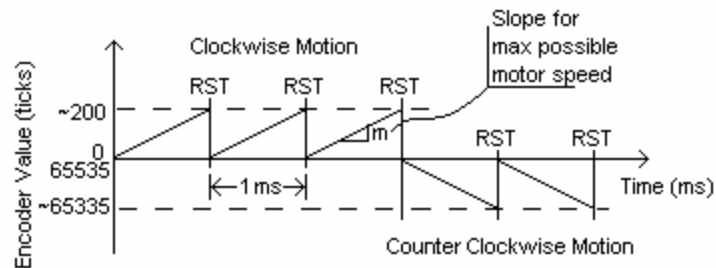
Figure 16. Value of 16-bit Encoder Count During Motor Operation in Configuration A (Count is read just prior to Reset, RST)
