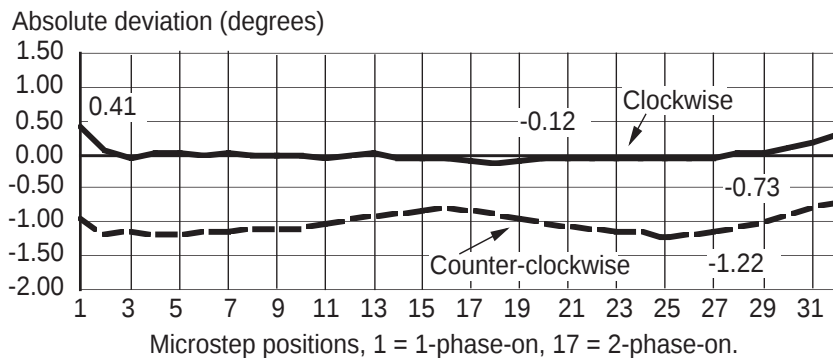
Figure 14. Sine/cosine compensated microstepping position ripple for a 57mm 7.5° PM stepper. CW ripple = 0.41 - (-0.12) = 0.53 degrees = 7% compared to 22% for uncompensated.
