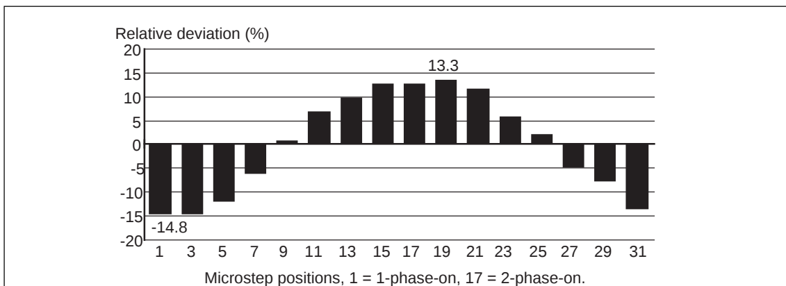
Figure 8. Microstepping holding torque ripple for a 57mm PM stepper. Ripple = 13.3 - (-14.8) = 28.1\% .
