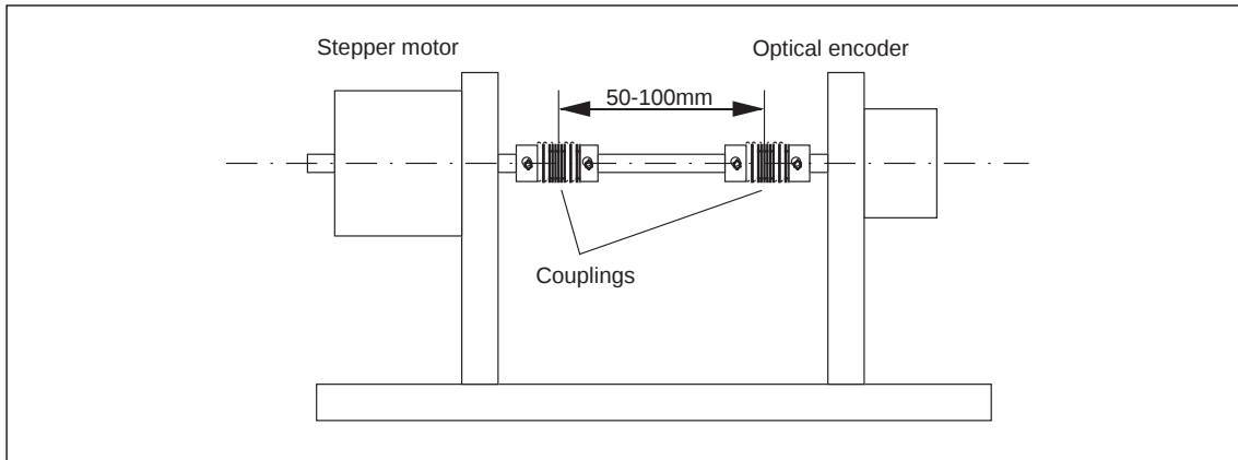
Figure 10. Suggested set-up for measuring microstepping position ripple.
