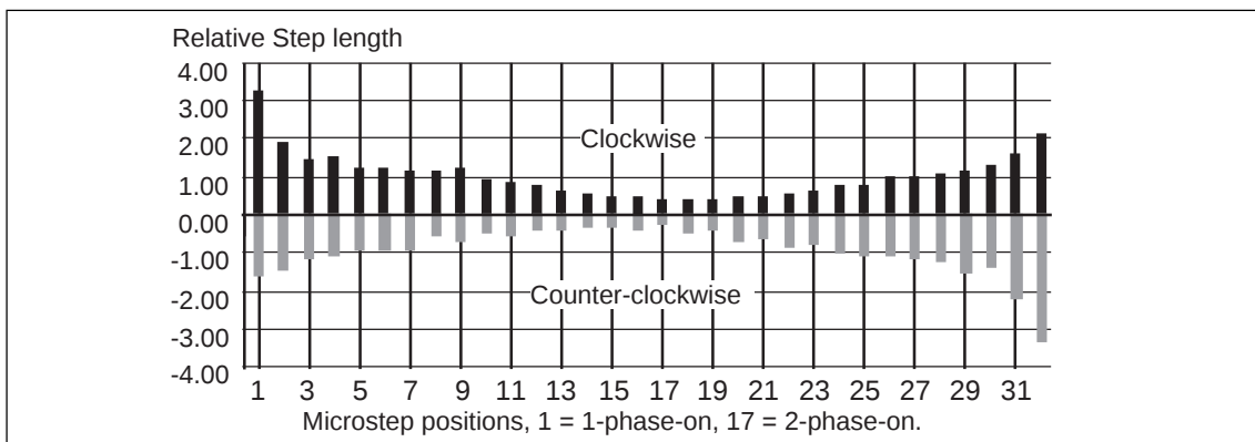
Figure 7. 57mm PM-stepper relative microstep length as function of stop position, 1/32 - full-step mode.
