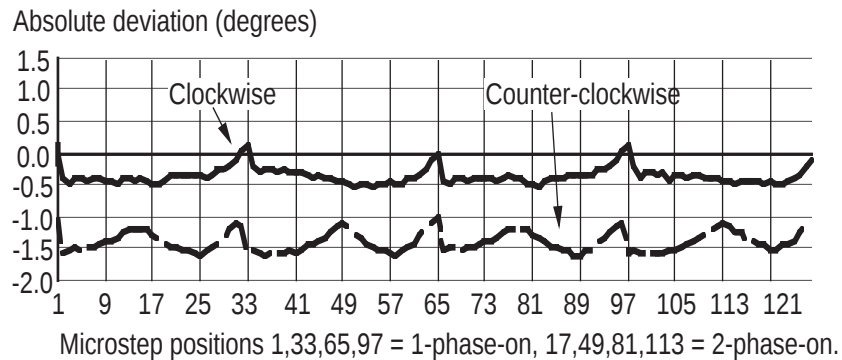
Figure 13. Sine/cosine CW compensated microstepping position ripple for 4 full-step cycles for a 57mm 7.5 degree PM stepper.
