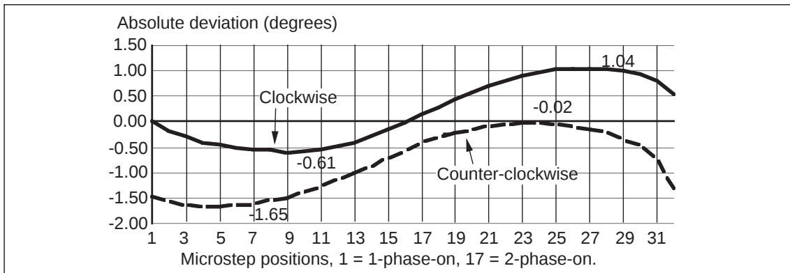
Figure 6. Microstepping position ripple for a 57mm 7.5 degree PM stepper. CW ripple = 1.04 - (-0.61) = 1.65 degrees = 22%.
