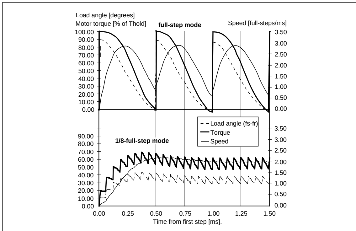
Figure 1. (A)—torque and speed ripple as function of load angle, full-step mode.
