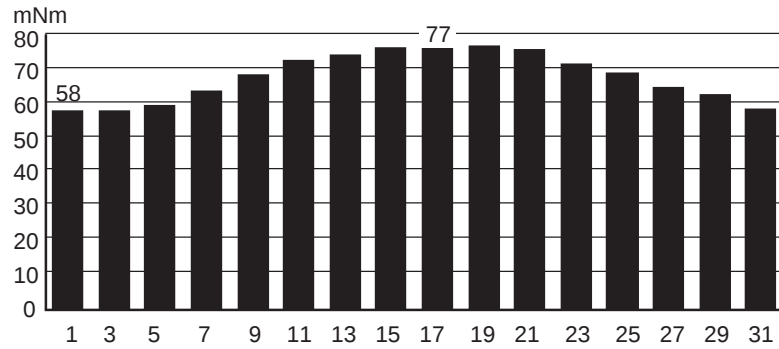
Figure 12. Microstepping holding torque for a 57mm PM stepper.
