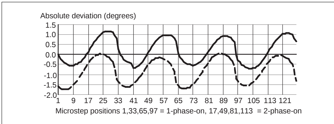
Figure 11. Microstepping position ripple for 4 full-step cycles for a 57mm 7.5 degree PM stepper.
