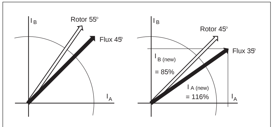
Figure 5. (A)—rotor and flux directions at original full-step position. (B)—rotor and flux directions at adjusted full-step position.
