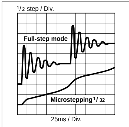
Figure 4. Rotor position as function of stepping mode.
