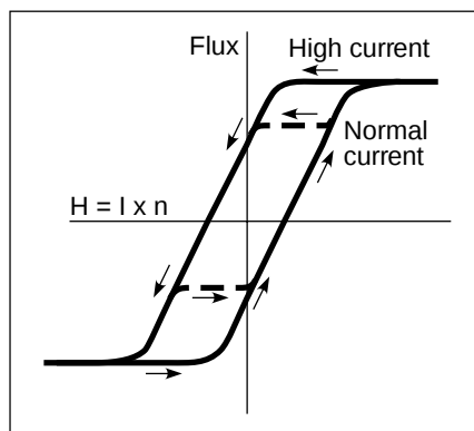
Figure 9. Flux as function of flux history and H-value when two different current levels are applied to the winding.
