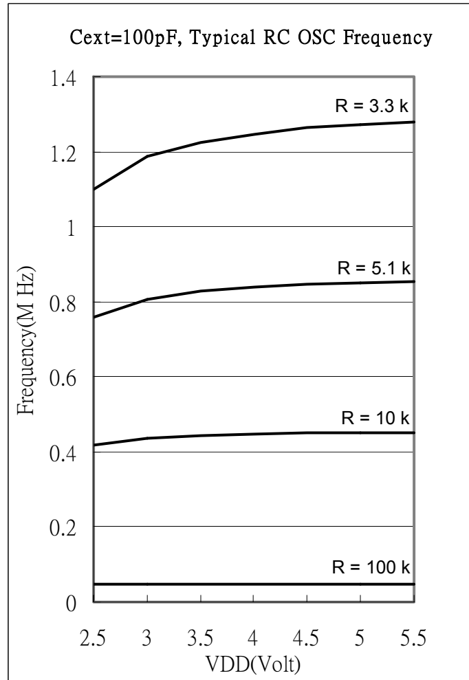
Fig. 35 Typical RC OSC Frequency vs. VDD (Cext=100pF, Temperature at 25 °C)
