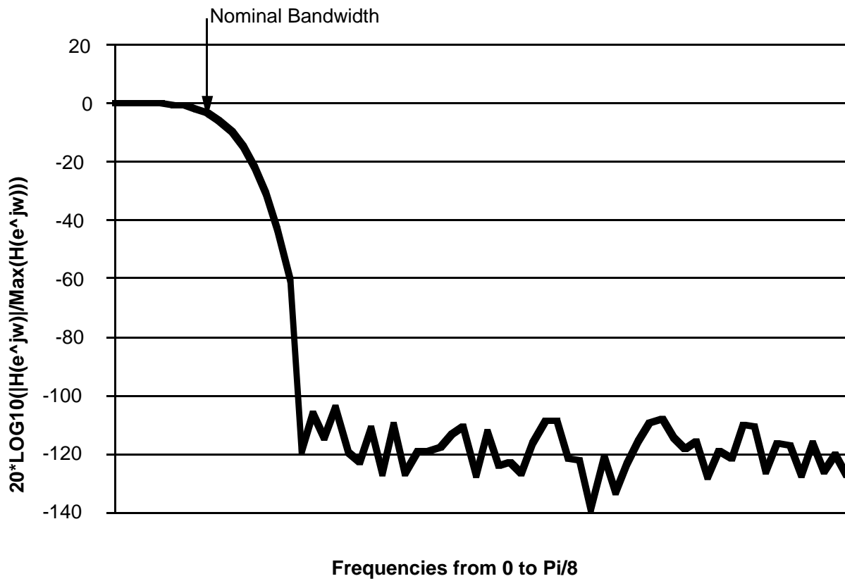
Figure 6 Frequency Response of Prototype Filter, h[n]
