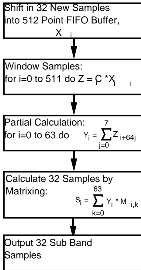
Figure 4 Flow Diagram of the MPEG/Audio Encoder Filter Bank
