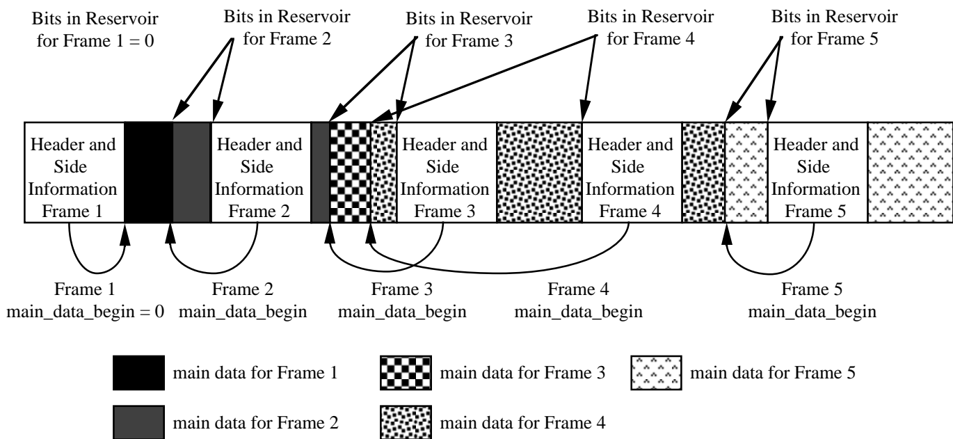
Figure 22 Layer III Bitstream Digram
