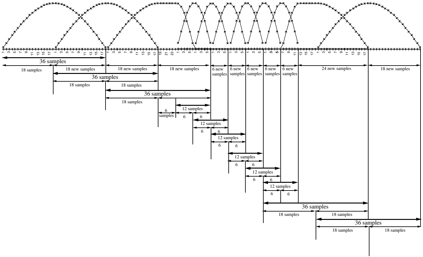
Figure 21 The Arrangement of Overlapping MDCT Windows
