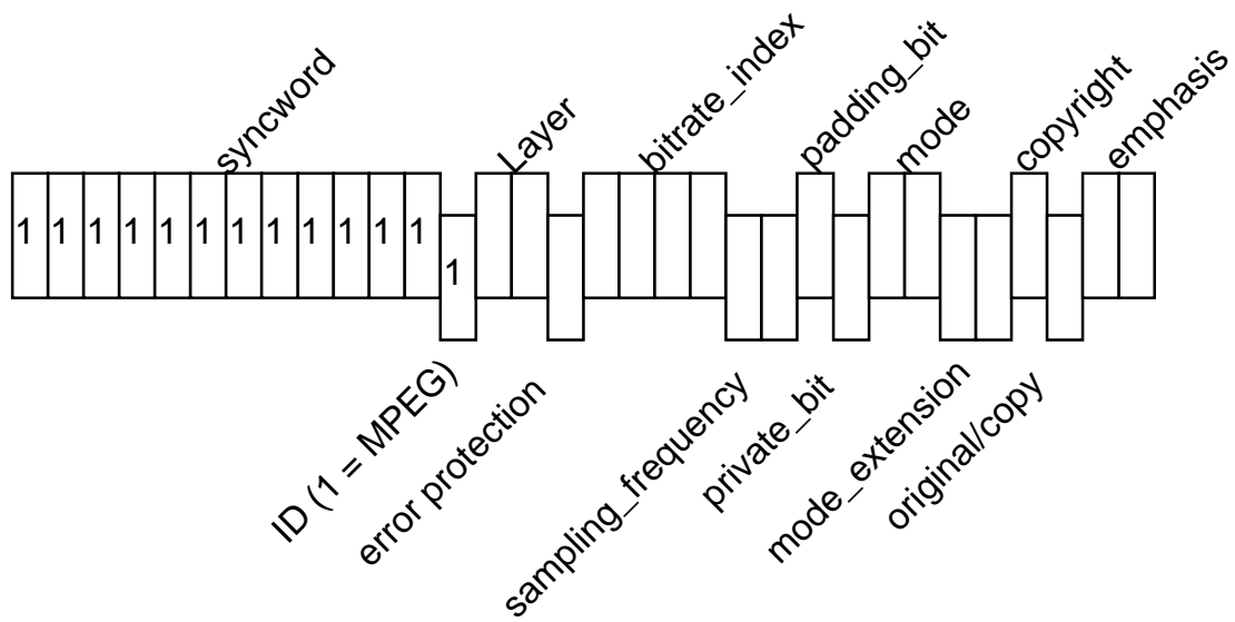
Figure 17 MPEG Header Syntax
