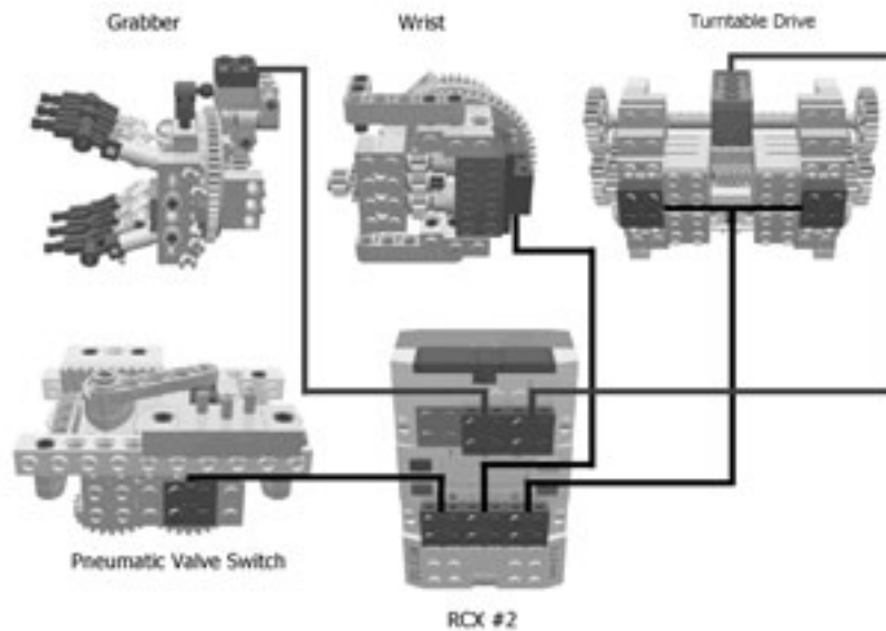
Figure 7.13 System Schematic for RCX 2
