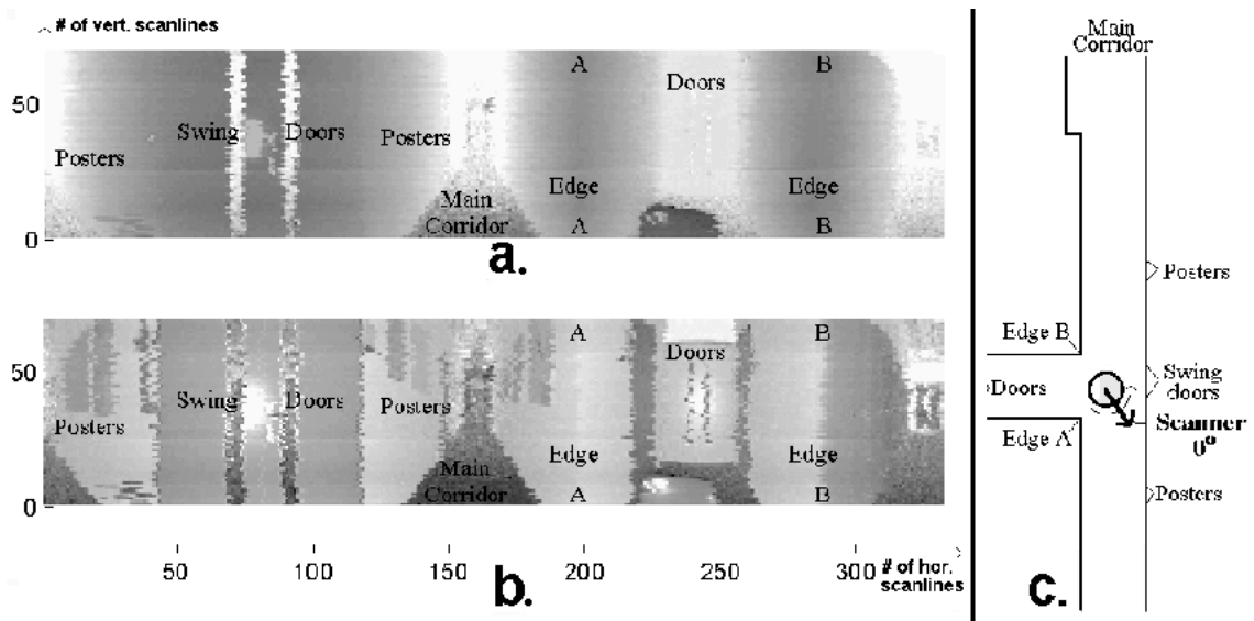
Figure 4.31: Range and intensity scans obtained with Adams' 3-D Imaging Scanner.
