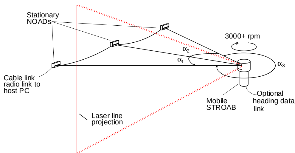
Figure 6.21: The Computerized Opto-electronic Navigation and Control (CONAC TM ) system employs an onboard, rapidly rotating and vertically spread laser beam, which sequentially contacts the networked detectors. (Courtesy of MTI Research, Inc.)
