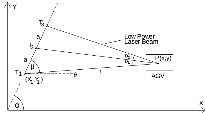
Figure 6.18: Three equidistant collinear photosensors are employed in lieu of retroreflective beacons in the Imperial College laser triangulation system for AGV guidance. (Adapted from [Premi and Besant, 1983].)
