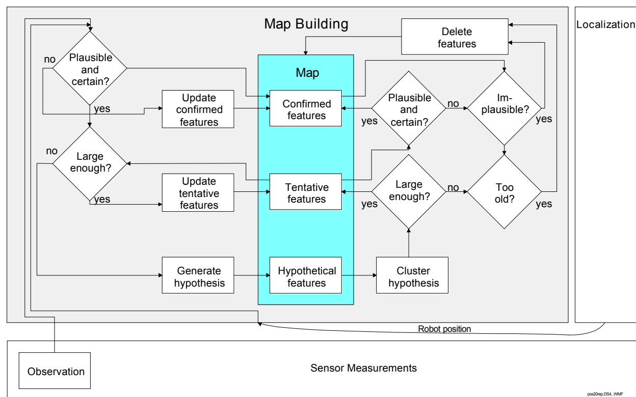
Figure 8.8: The basic map-building algorithm maintains a hypothesis tree for the three sensor reading categories: hypothetical, tentative, and confirmed. (Adapted from [Rencken, 1994].)
