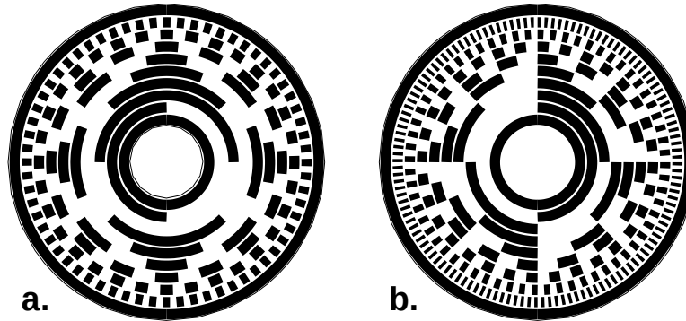
Figure 1.3: Rotating an 8-bit absolute Gray code disk.
