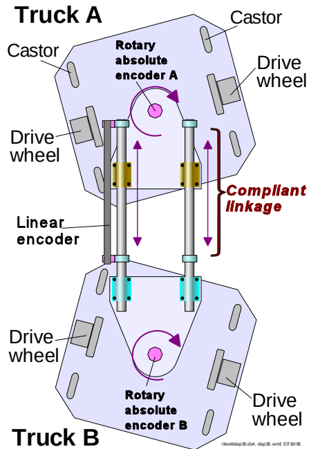
Figure 1.15: The compliant linkage is instrumented with two absolute rotary encoders and a linear encoder to measure the relative orientations and separation distance between the two trucks.
