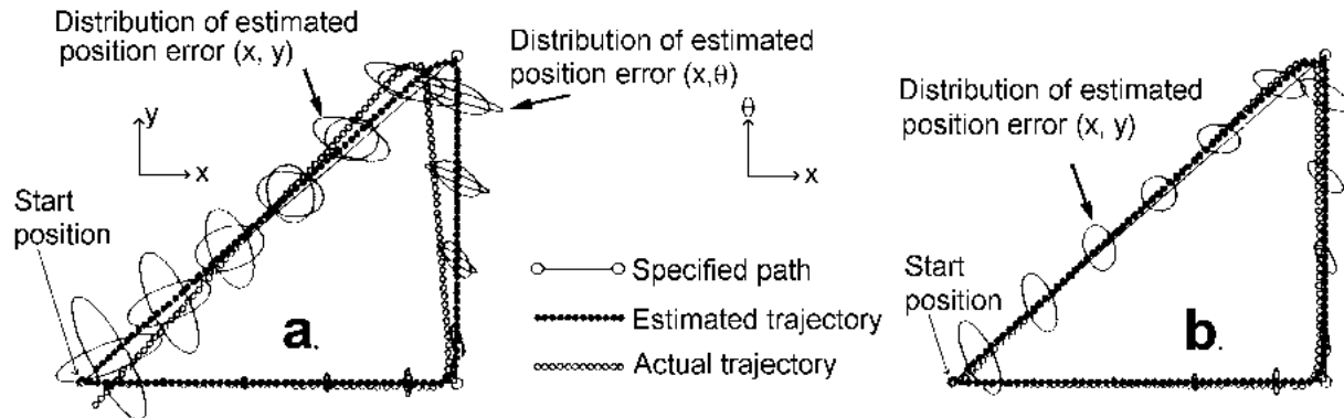
Figure 5.15: Computer simulation of a mobile robot run.. (Adapted from [Komoriya and Oyama, 1994].)
