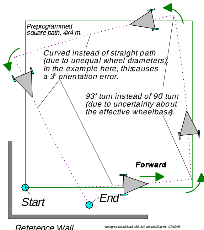
Figure 5.4: The effect of the two dominant systematic odometry errors E_b and E_d : when the square path is performed in the opposite direction one may find that the errors add up.
