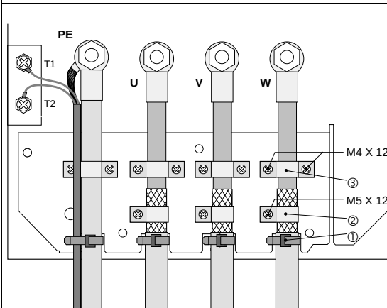
FIG 4-17 Proposal for motor connection with 822X
