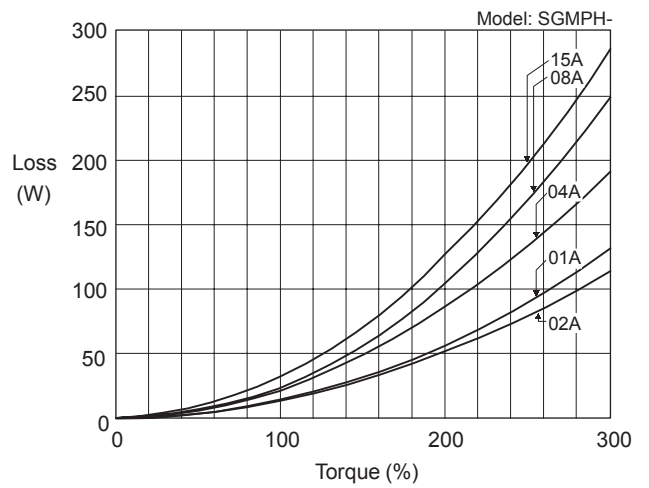
SGMPH Servomotors
