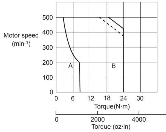
SGMCS-25D
