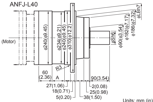
ANFJ-L40
