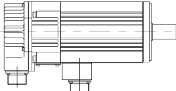
Servomotor-end connector
