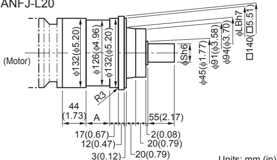
ANFJ-L20
