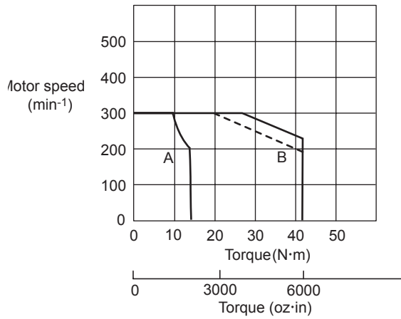
SGMCS-17D
