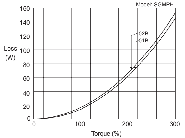
SGMPH Servomotors
