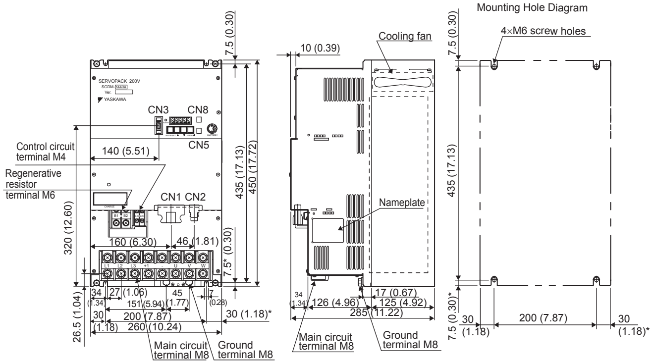
View A
