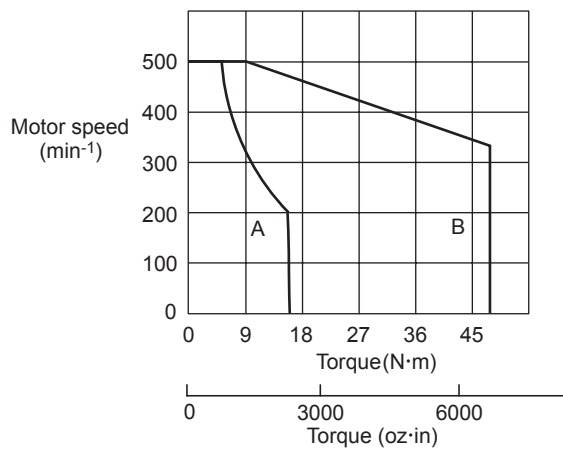
SGMCS-16E
