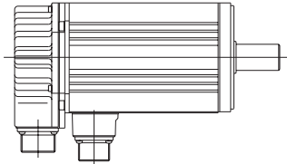
Servomotor-end connector
