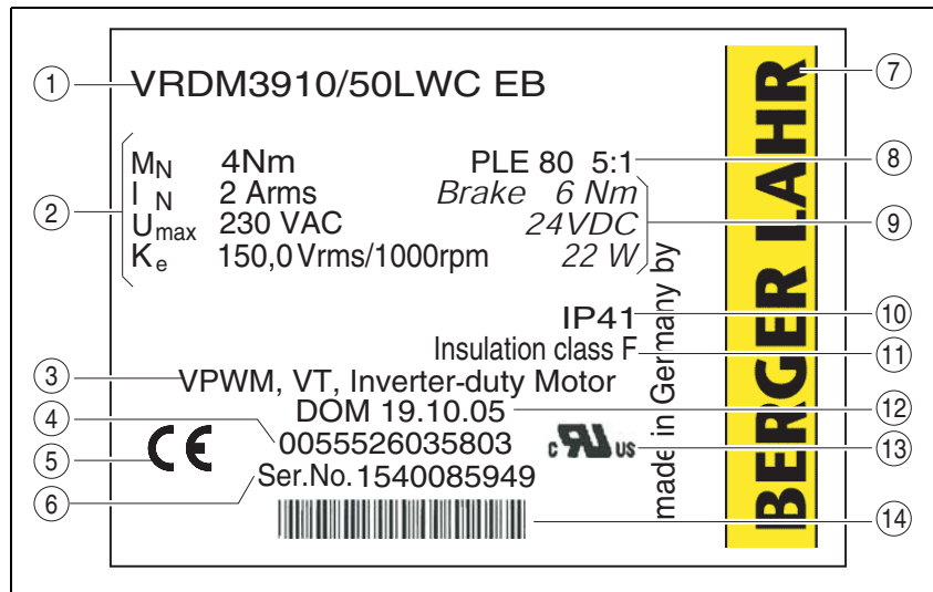
Figure 1.1 Name plate
