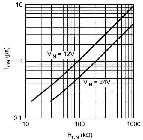
T_{ON} vs R_{ON} , LM3404 ( T_A = 25^\circ\text{C} )
