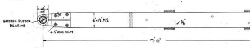
ASSEMBLY 1 1/2" = 1 FT
