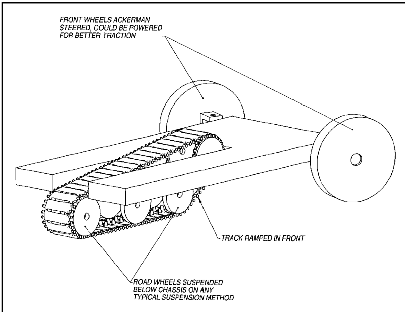
Figure 5-12 One track, two front wheels, Ackerman steer
