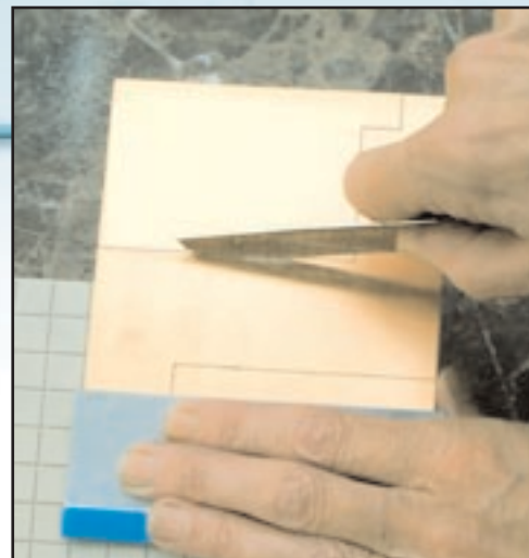
Cutting the endplates from the circuit board
